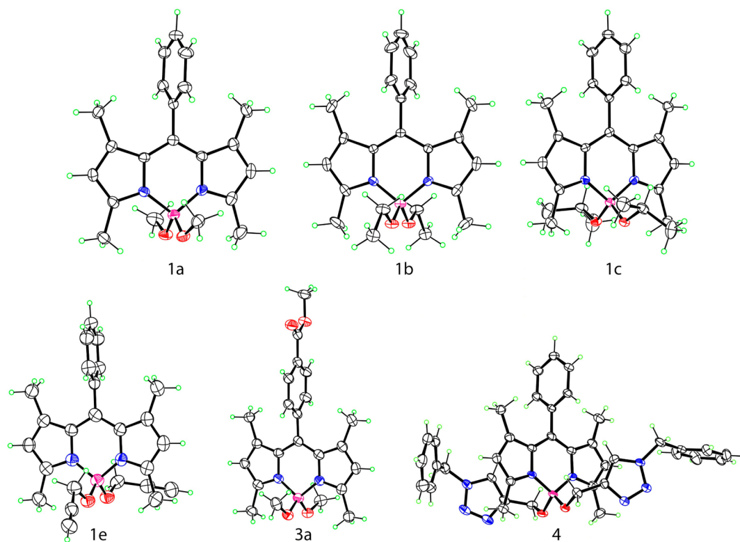
Figure 1. Molecular structures of BODIPYs 1a–c,e , 3a , and 4 from X-ray crystal structure analysis, with 50% probability ellipsoids. Only one of the independent molecules is shown for those structures with Z' > 1 .
