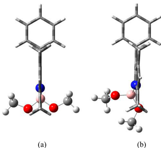
Figure 2. Molecular structures of (a) the symmetric conformer 1a and (b) the unsymmetric conformer 1a' from B3LYP/6-31+G(d,p) optimization.
