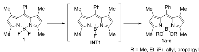
Scheme 2. Boronium Intermediate INT1 and BODIPYs 1a–e Formed using Methods B and C
